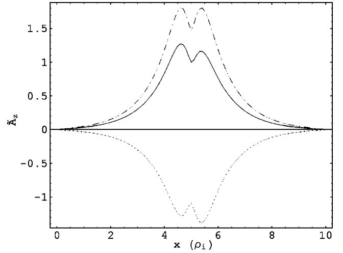
FIG. 2. \tilde{A}_z(x) as the eigenfunction. Solid line, the real part, dotted line, the imaginary part, and dashed line, the absolute value. Plot is scaled to the unit that \Re \tilde{A}_z(L_x/2) = 1 .
