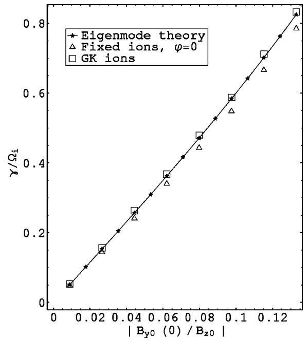
FIG. 5. Linear growth rate is proportional to amplitude of B_{y0} . L_x=L_y=10\rho_i , a=0.5\rho_i , and \beta=1\% . Amplitude of equilibrium current is varied to give different values of B_{y0} .
