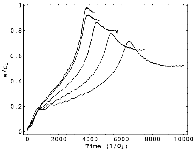
FIG. 9. Nonlinear evolution of the semicollisional tearing mode with different values of collision frequency. Same parameters as Fig. 8. \nu_c equals to 0.0005\Omega_i , 0.001\Omega_i , 0.002\Omega_i , 0.003\Omega_i , and 0.004\Omega_i for saturation levels from low to high, respectively.
